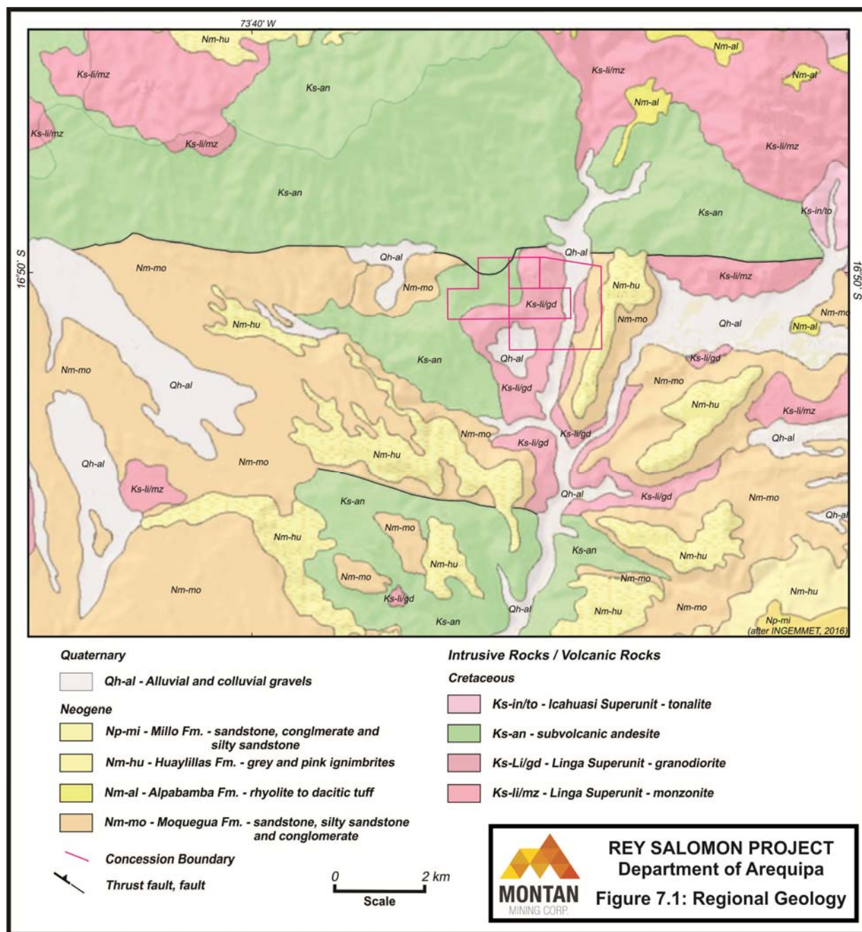
Figure 7.1: Regional Geologic Map for the Rey Salomon Property
